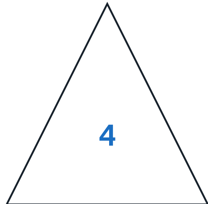
4. isosceles triangle
