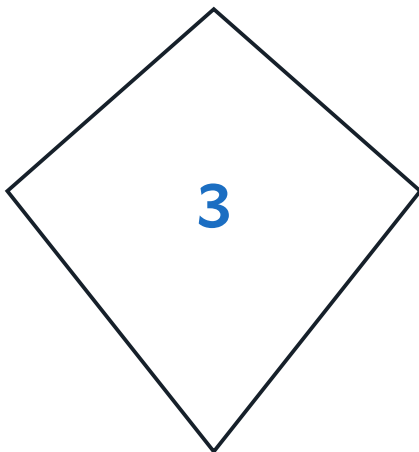
3. kite
