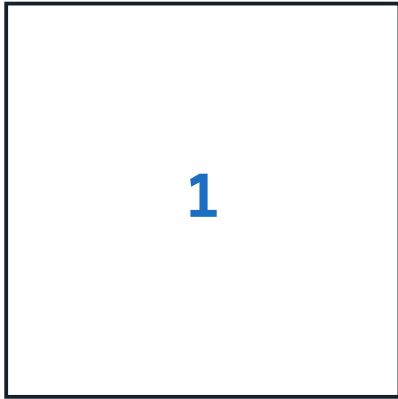
1. square
