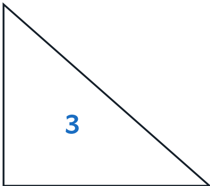
3. right scalene
