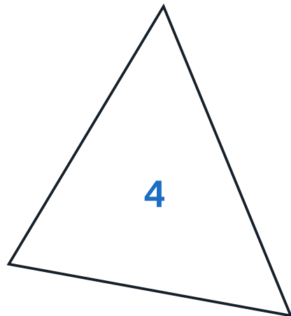
4. acute scalene
