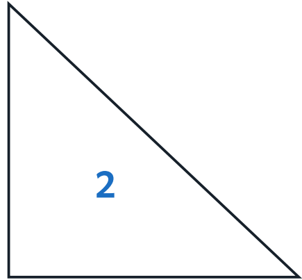
2. right-angled
